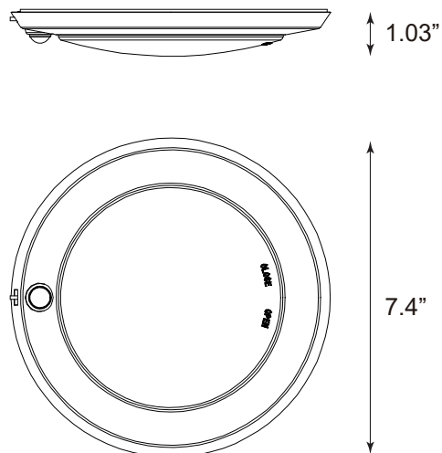
11-DK6-10L-KFS-OS
