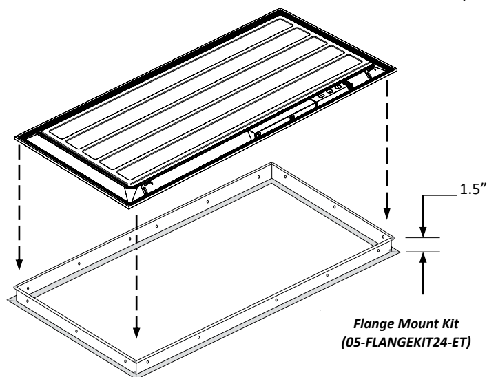
Surface Mounting Kit (05-SMKT-24S)
